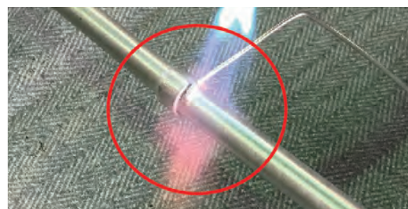
Change in flame color of preheated aluminum pipe
