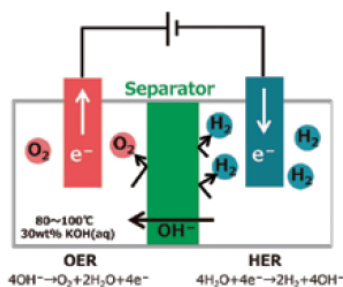
Image of alkaline water electrolysis
