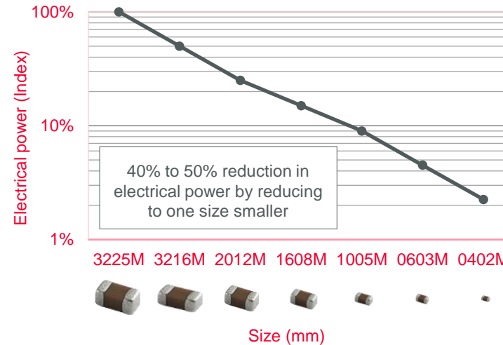
Reducing power used in manufacturing (MLCCs example)
